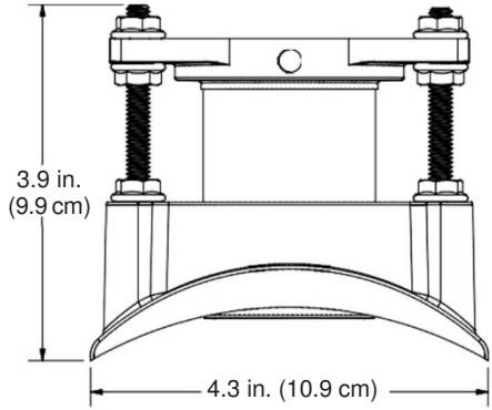
SADDLE – FRONT VIEW
