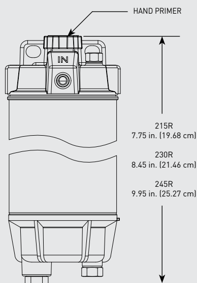
200 Series Front
